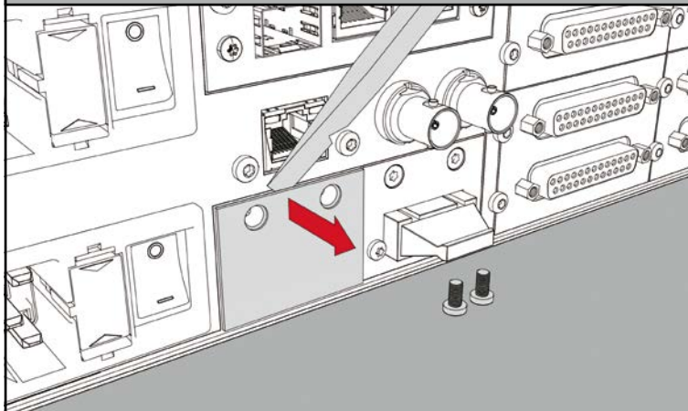
C Remove Cover Plate
